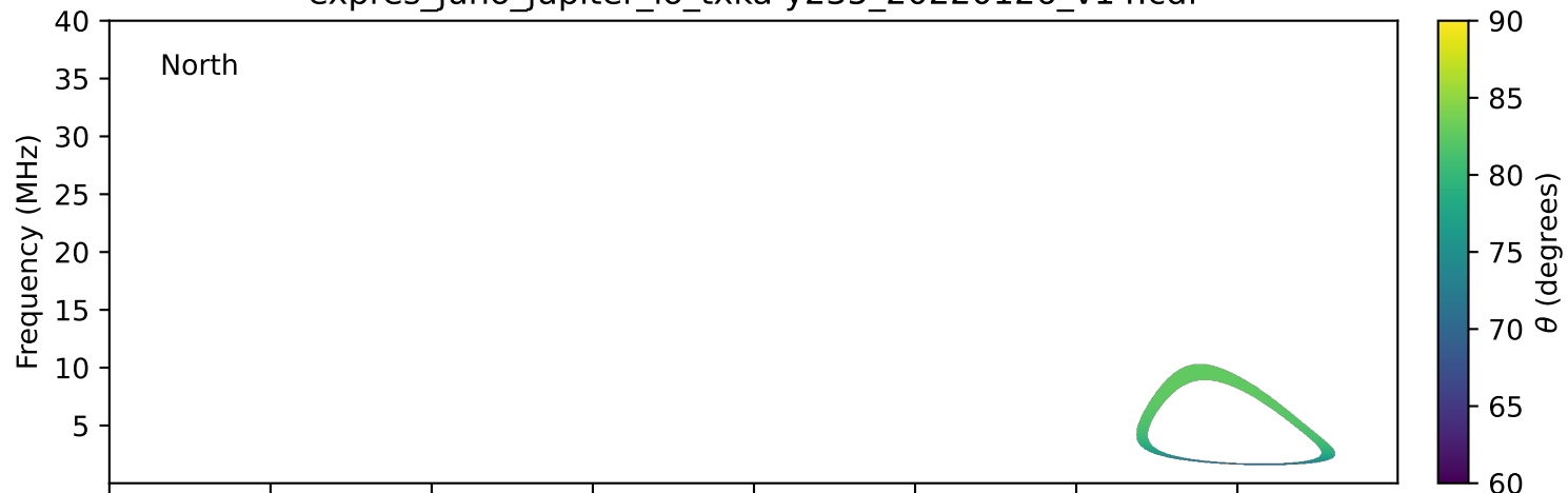
expres_juno_jupiter_io_txka-y235_20220126_v14.cdf
