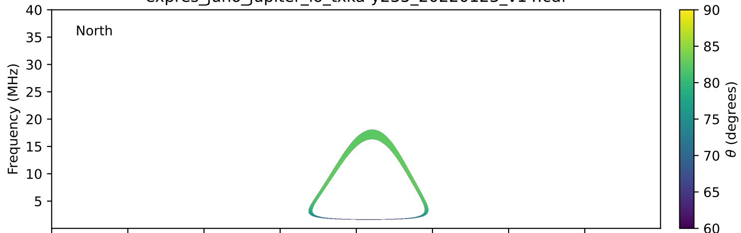
expres_juno_jupiter_io_txka-y235_20220123_v14.cdf
