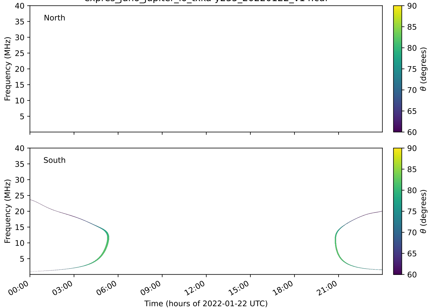
expres_juno_jupiter_io_txka-y235_20220122_v14.cdf
