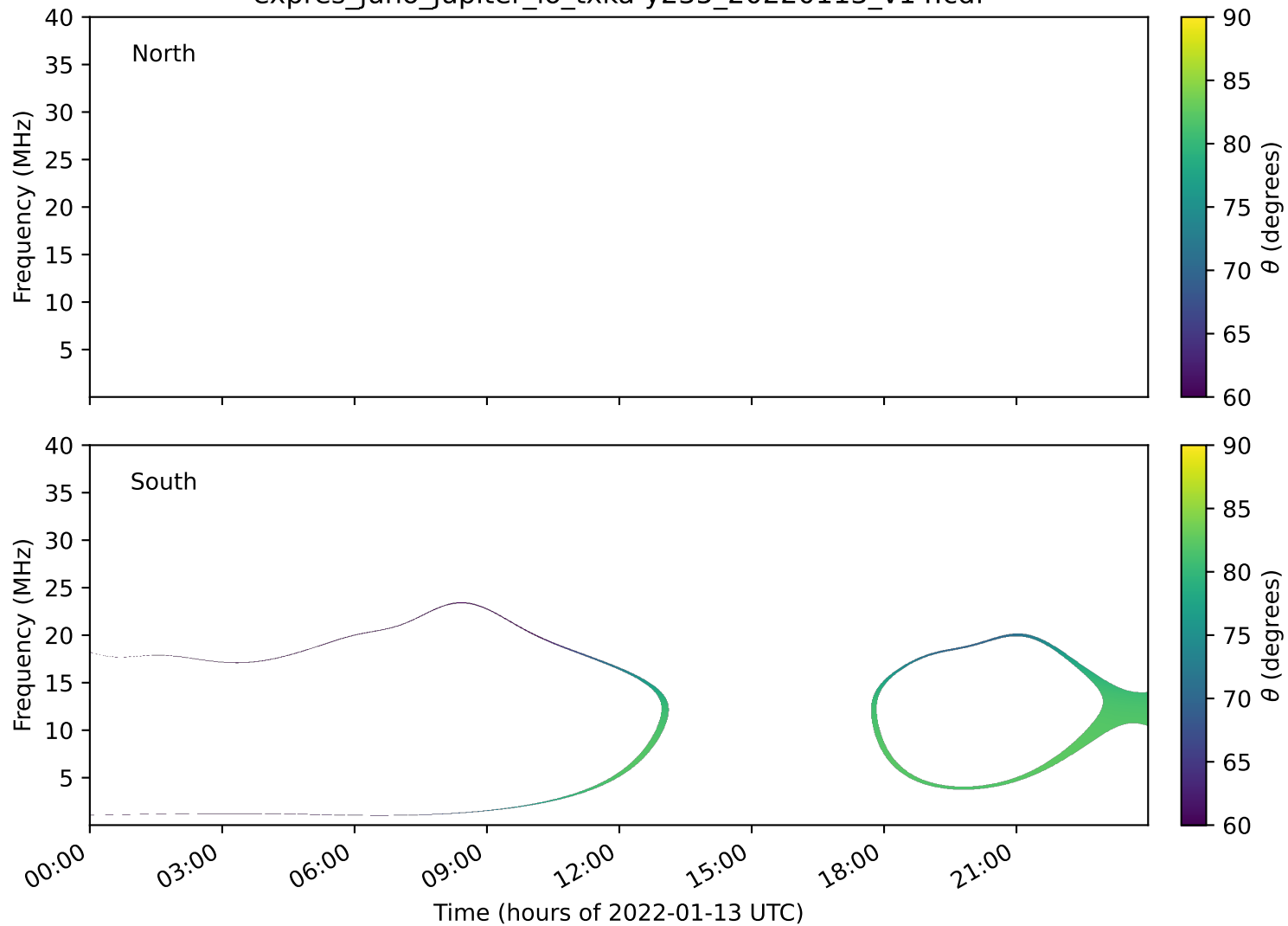
expres_juno_jupiter_io_txka-y235_20220113_v14.cdf
