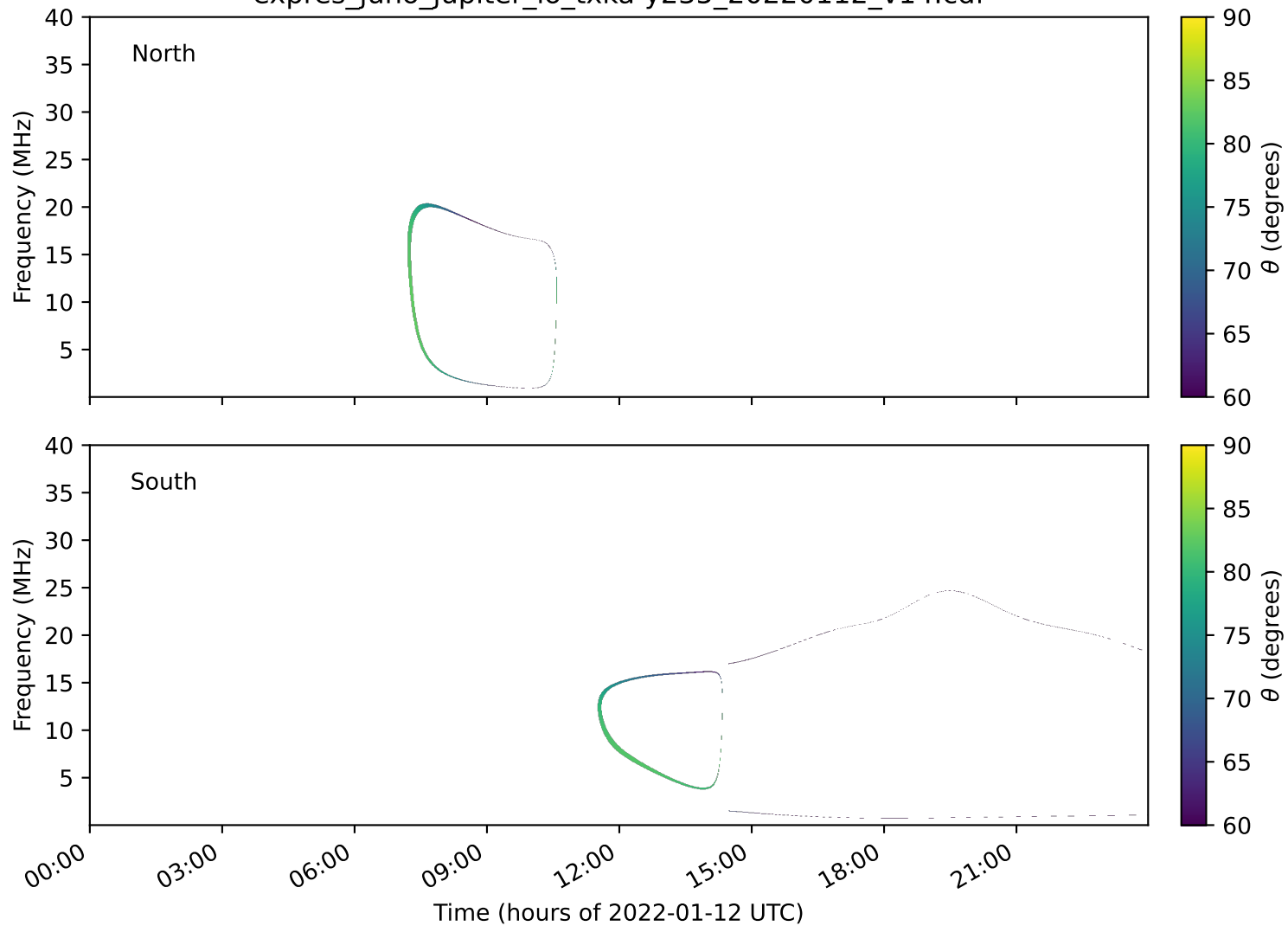
expres_juno_jupiter_io_txka-y235_20220112_v14.cdf
