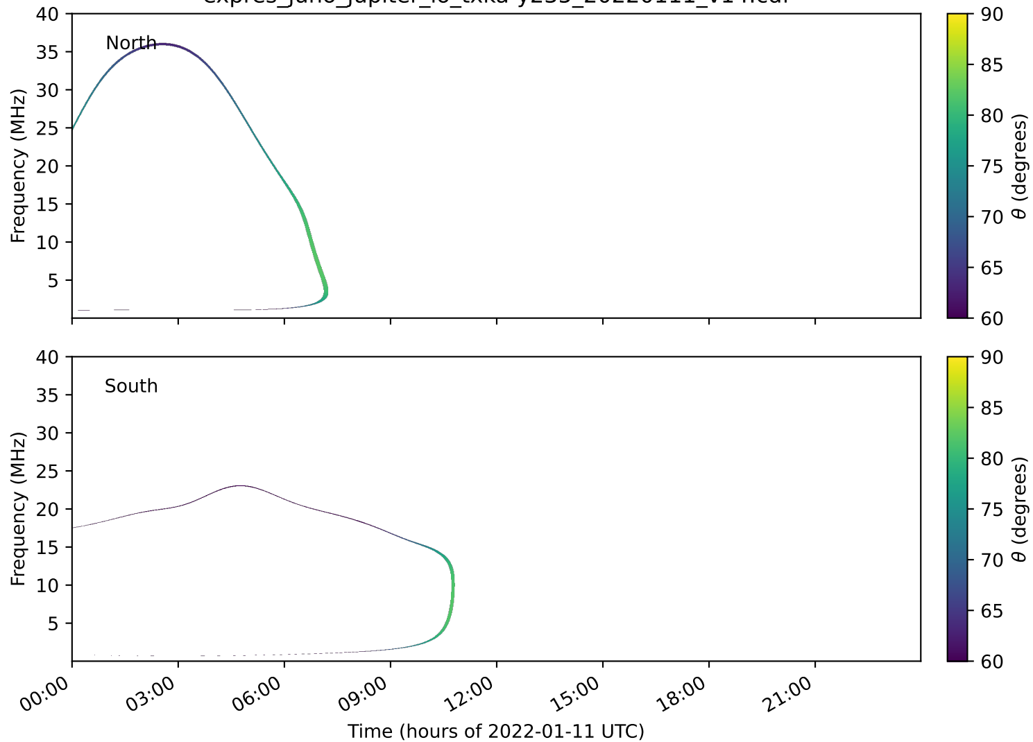
expres_juno_jupiter_io_txka-y235_20220111_v14.cdf
