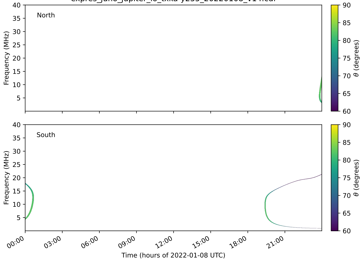
expres_juno_jupiter_io_txka-y235_20220108_v14.cdf
