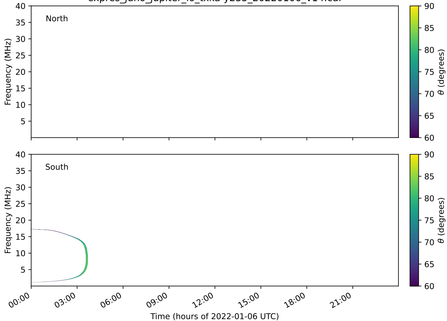
expres_juno_jupiter_io_txka-y235_20220106_v14.cdf
