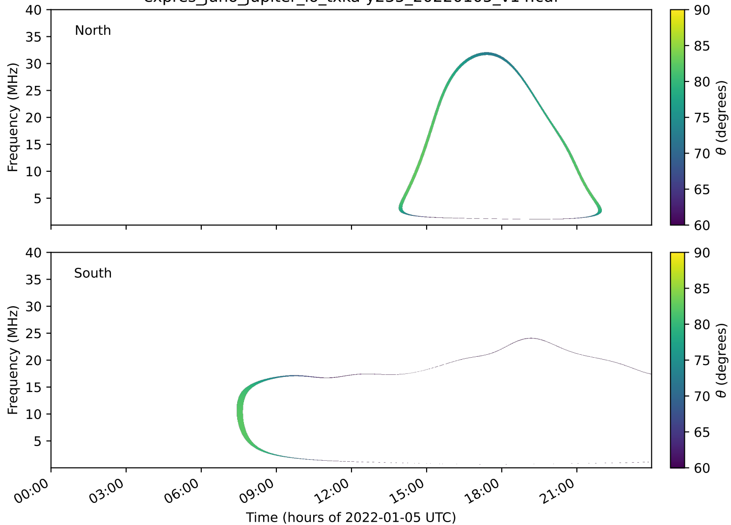
expres_juno_jupiter_io_txka-y235_20220105_v14.cdf
