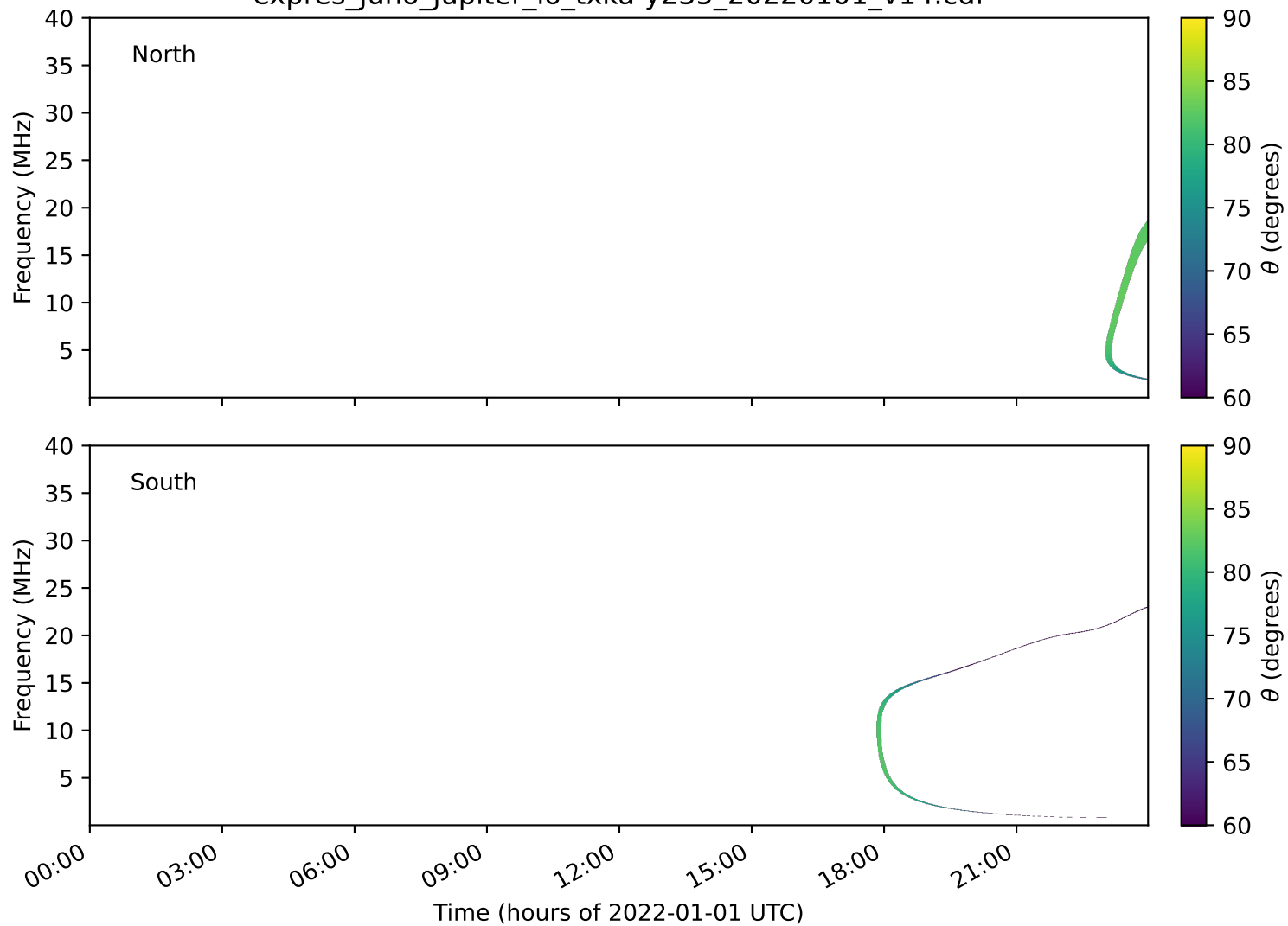
expres_juno_jupiter_io_txka-y235_20220101_v14.cdf
