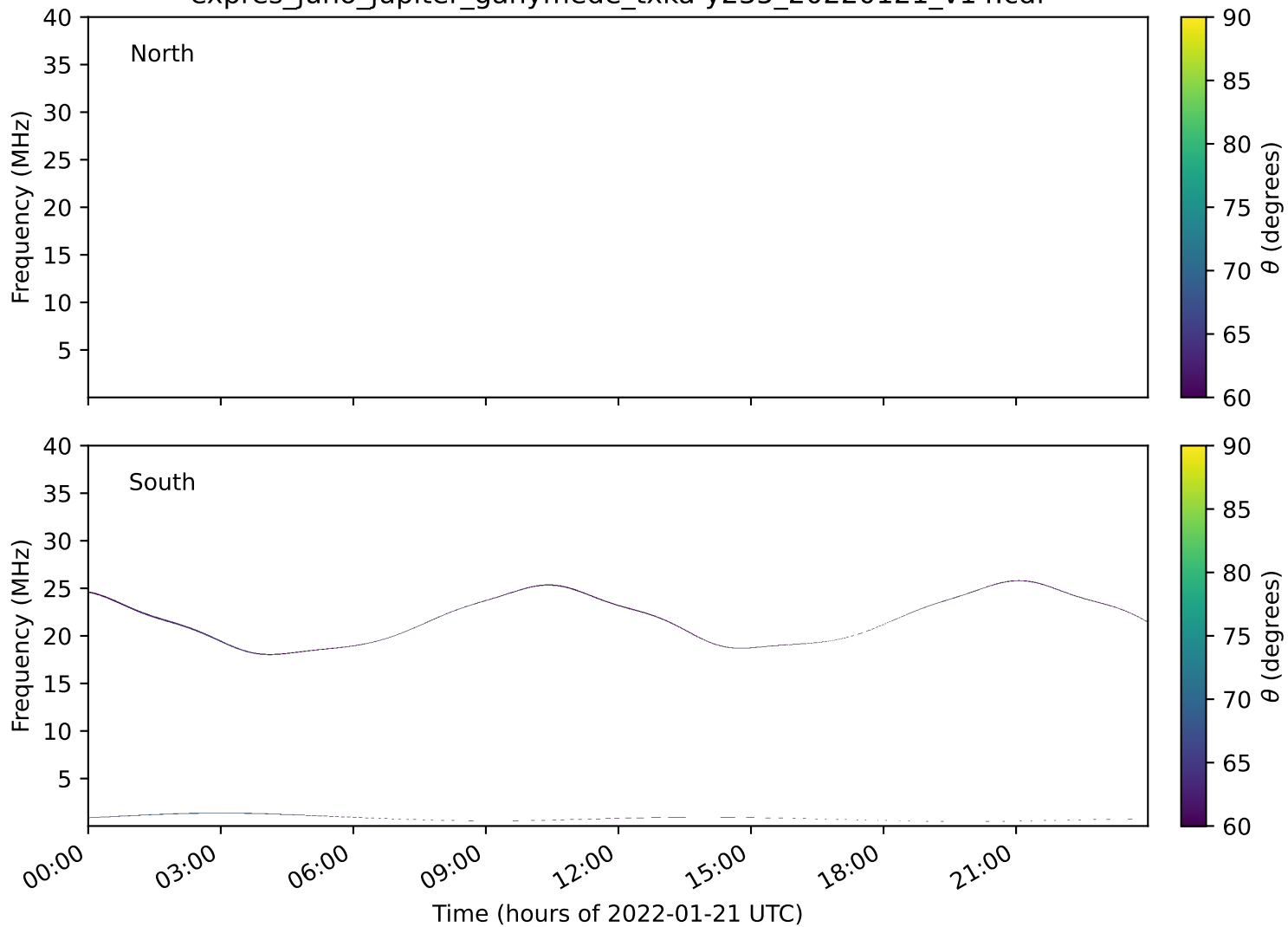
expres_juno_jupiter_ganymede_txka-y235_20220121_v14.cdf
