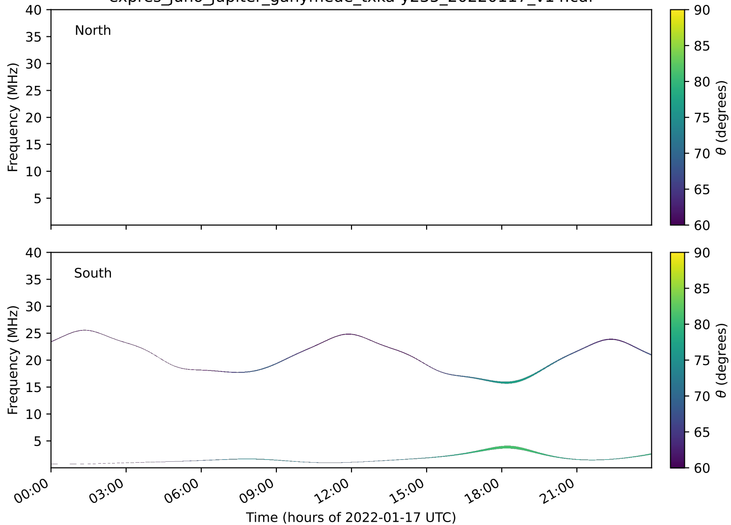
expres_juno_jupiter_ganymede_txka-y235_20220117_v14.cdf
