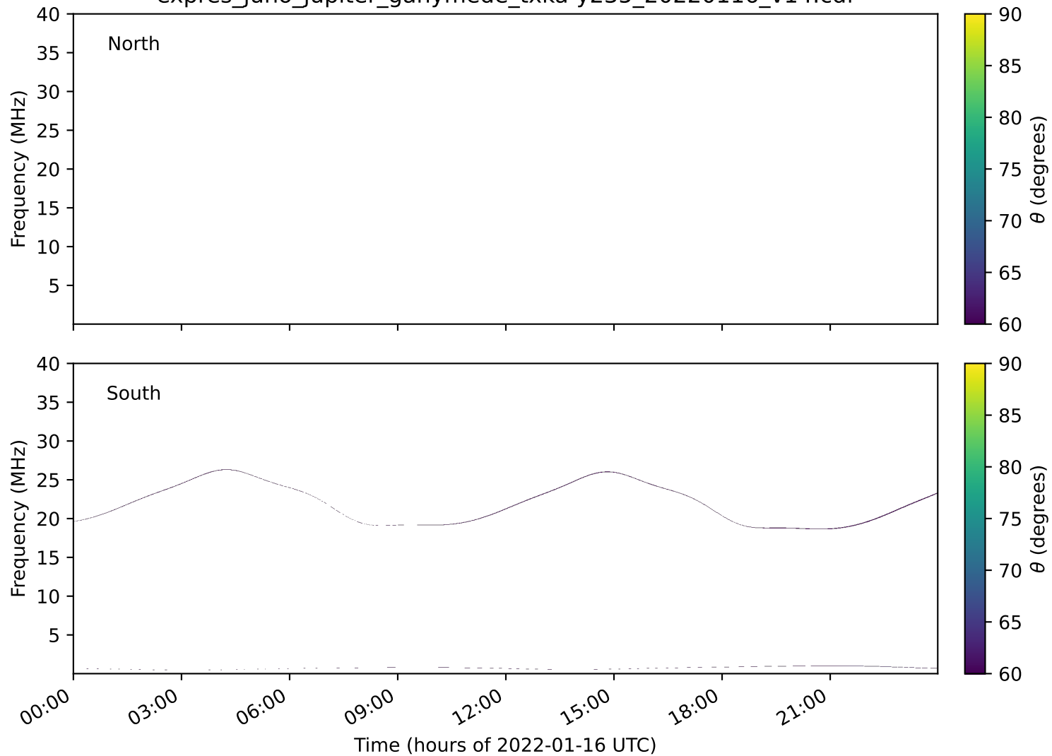
expres_juno_jupiter_ganymede_txka-y235_20220116_v14.cdf
