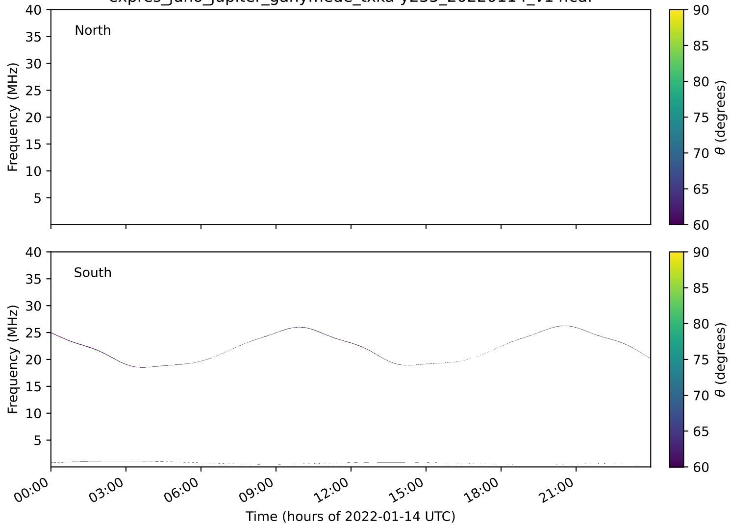
expres_juno_jupiter_ganymede_txka-y235_20220114_v14.cdf
