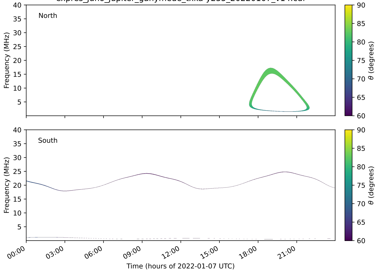
expres_juno_jupiter_ganymede_txka-y235_20220107_v14.cdf
