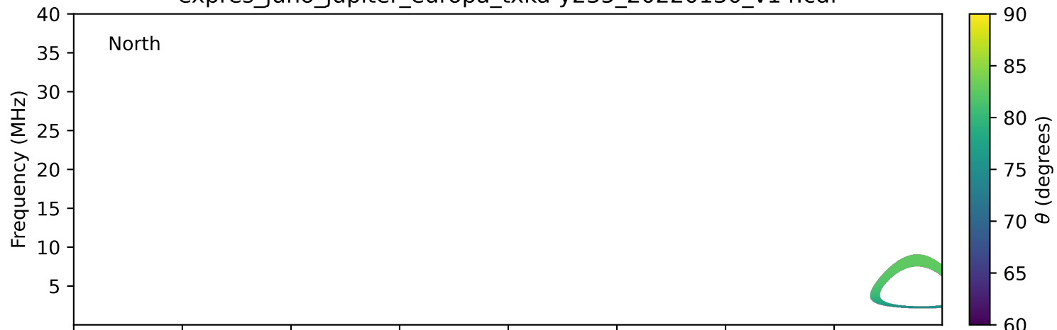
expres_juno_jupiter_europa_txka-y235_20220130_v14.cdf
