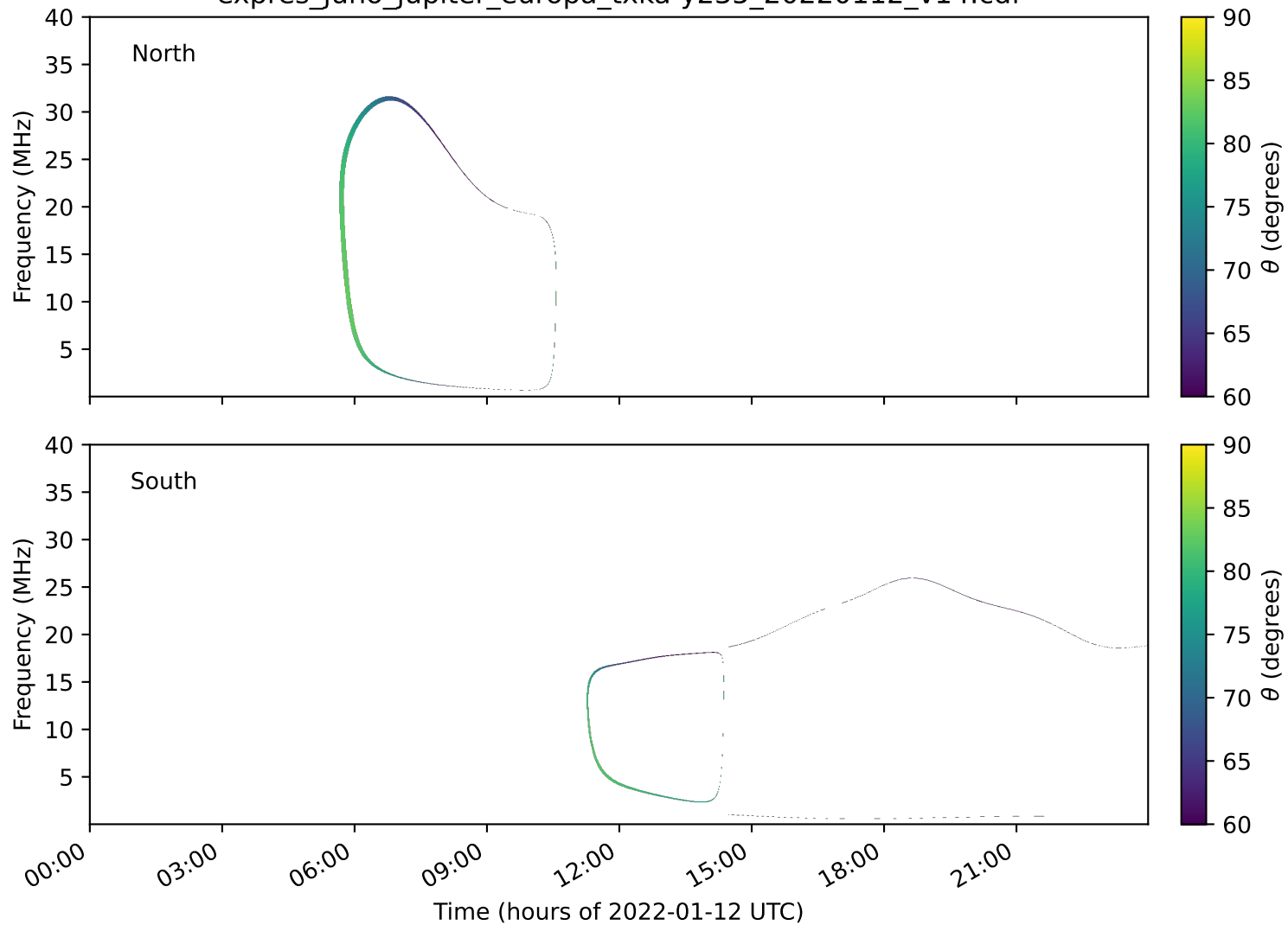
expres_juno_jupiter_europa_txka-y235_20220112_v14.cdf
