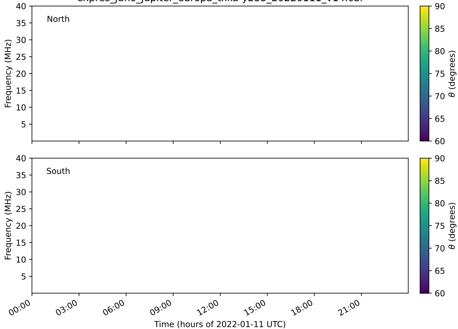
expres_juno_jupiter_europa_txka-y235_20220111_v14.cdf
