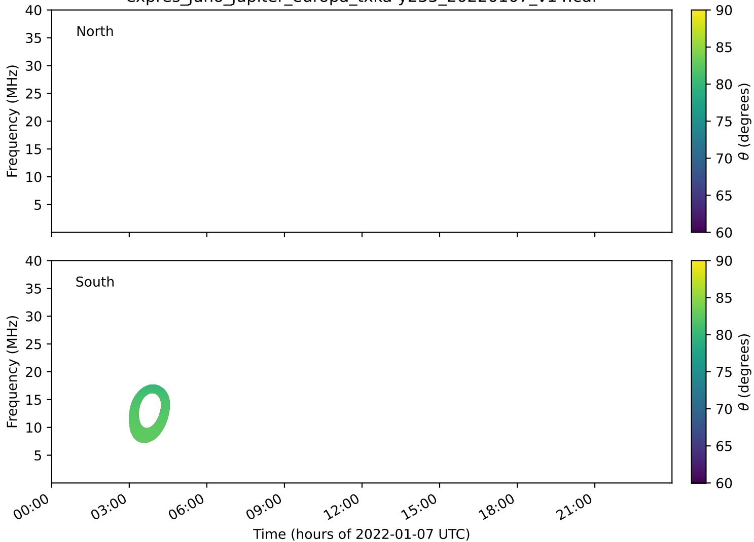
expres_juno_jupiter_europa_txka-y235_20220107_v14.cdf
