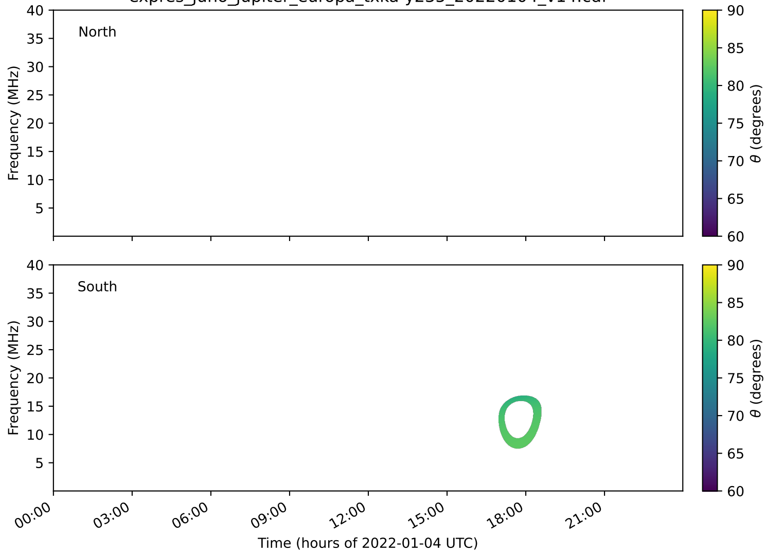
expres_juno_jupiter_europa_txka-y235_20220104_v14.cdf
