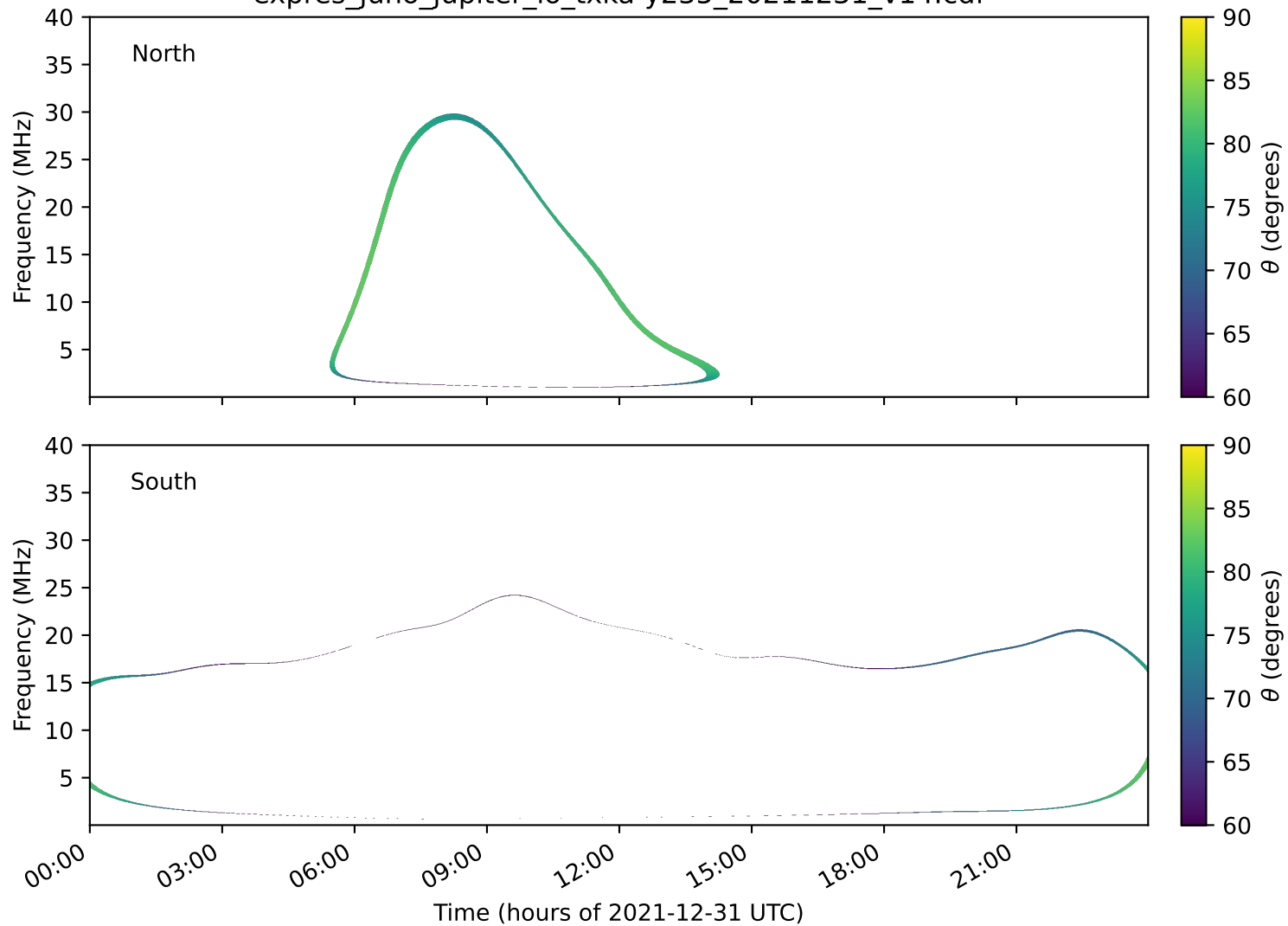
expres_juno_jupiter_io_txka-y235_20211231_v14.cdf
