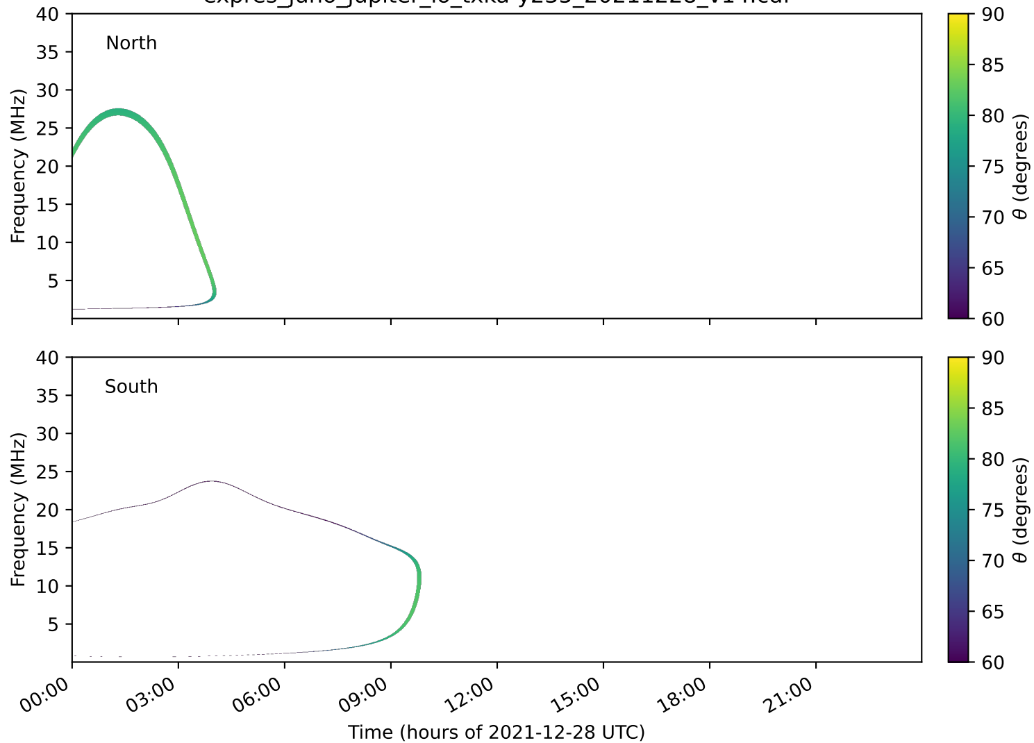
expres_juno_jupiter_io_txka-y235_20211228_v14.cdf
