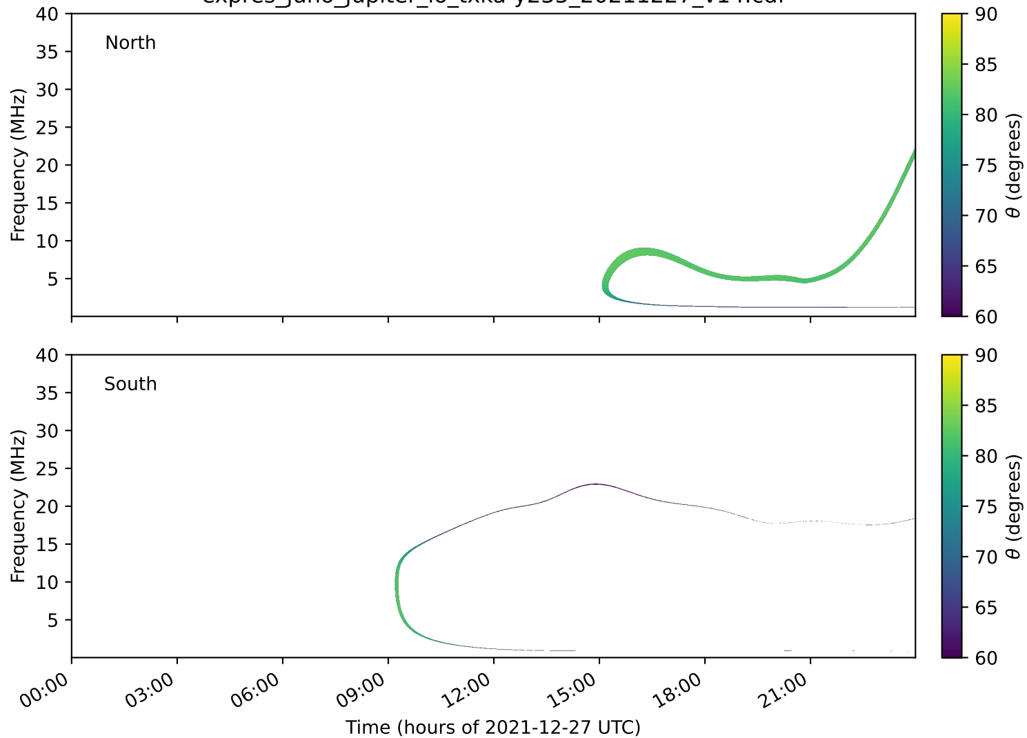
expres_juno_jupiter_io_txka-y235_20211227_v14.cdf
