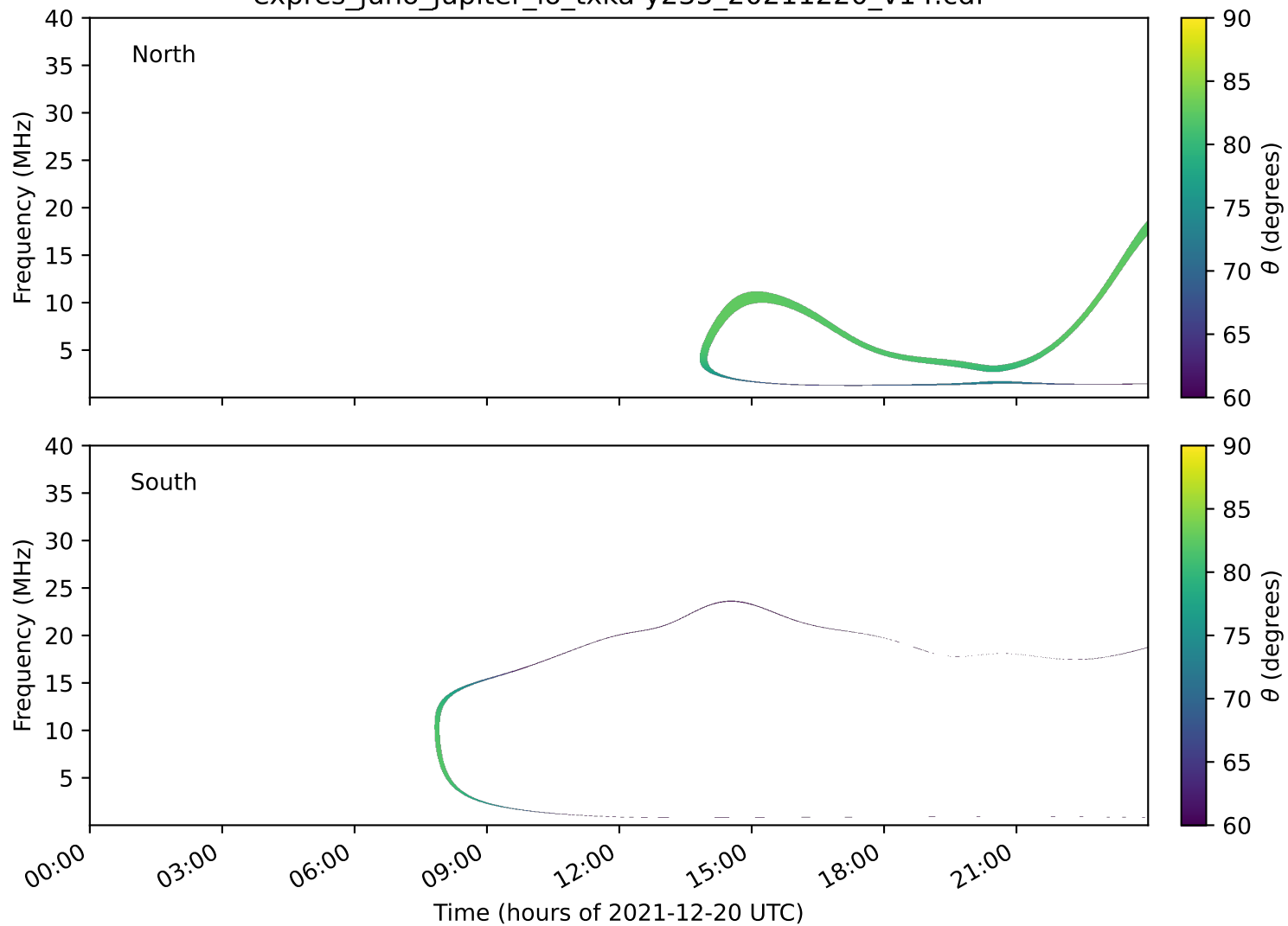
expres_juno_jupiter_io_txka-y235_20211220_v14.cdf
