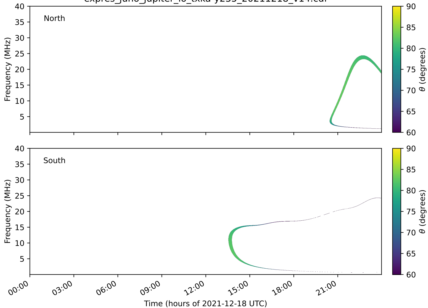
expres_juno_jupiter_io_txka-y235_20211218_v14.cdf
