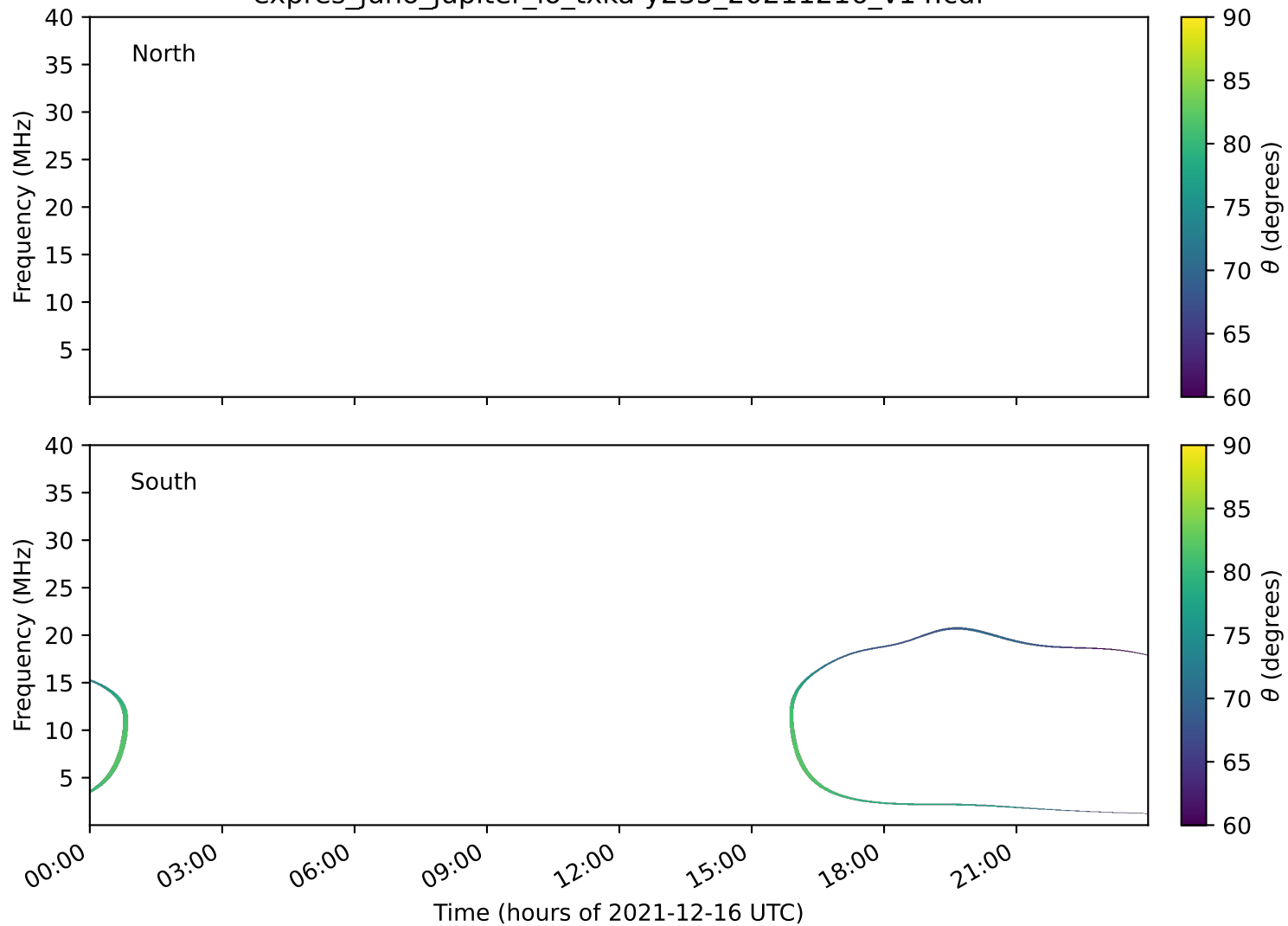
expres_juno_jupiter_io_txka-y235_20211216_v14.cdf
