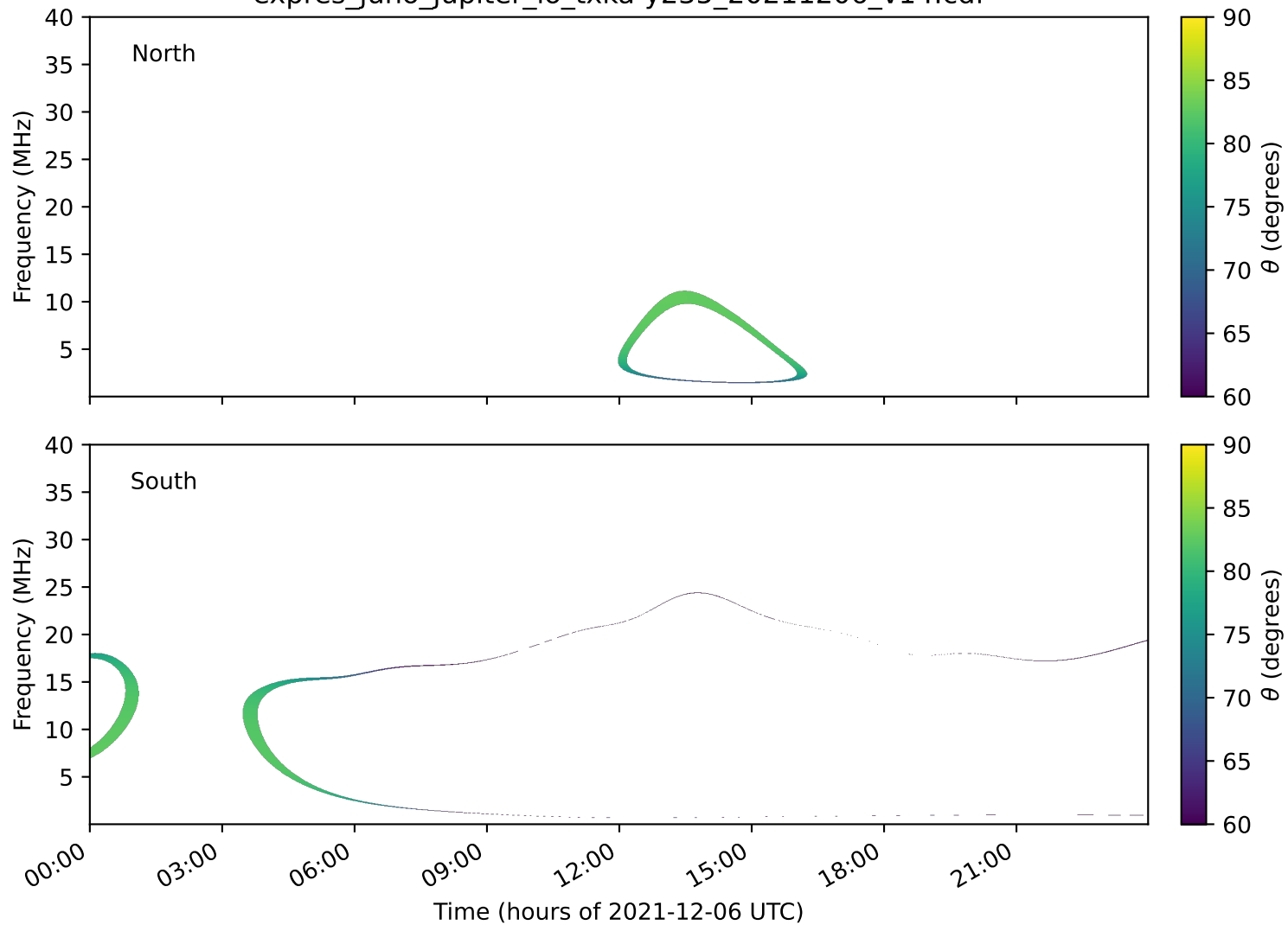
expres_juno_jupiter_io_txka-y235_20211206_v14.cdf
