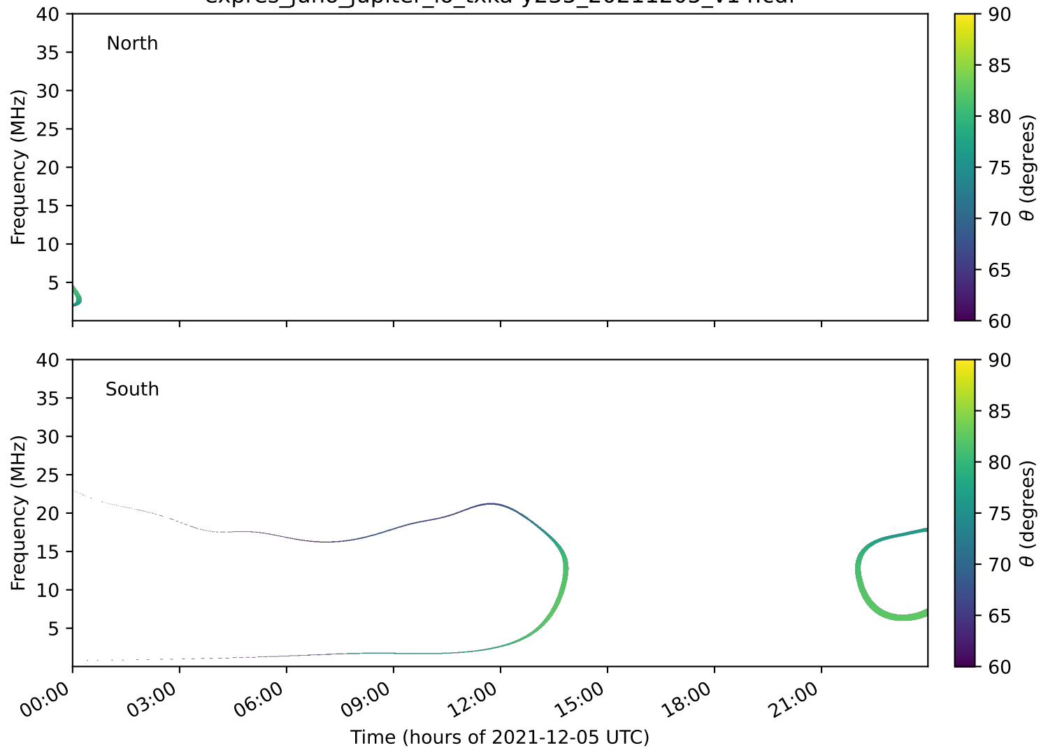
expres_juno_jupiter_io_txka-y235_20211205_v14.cdf
