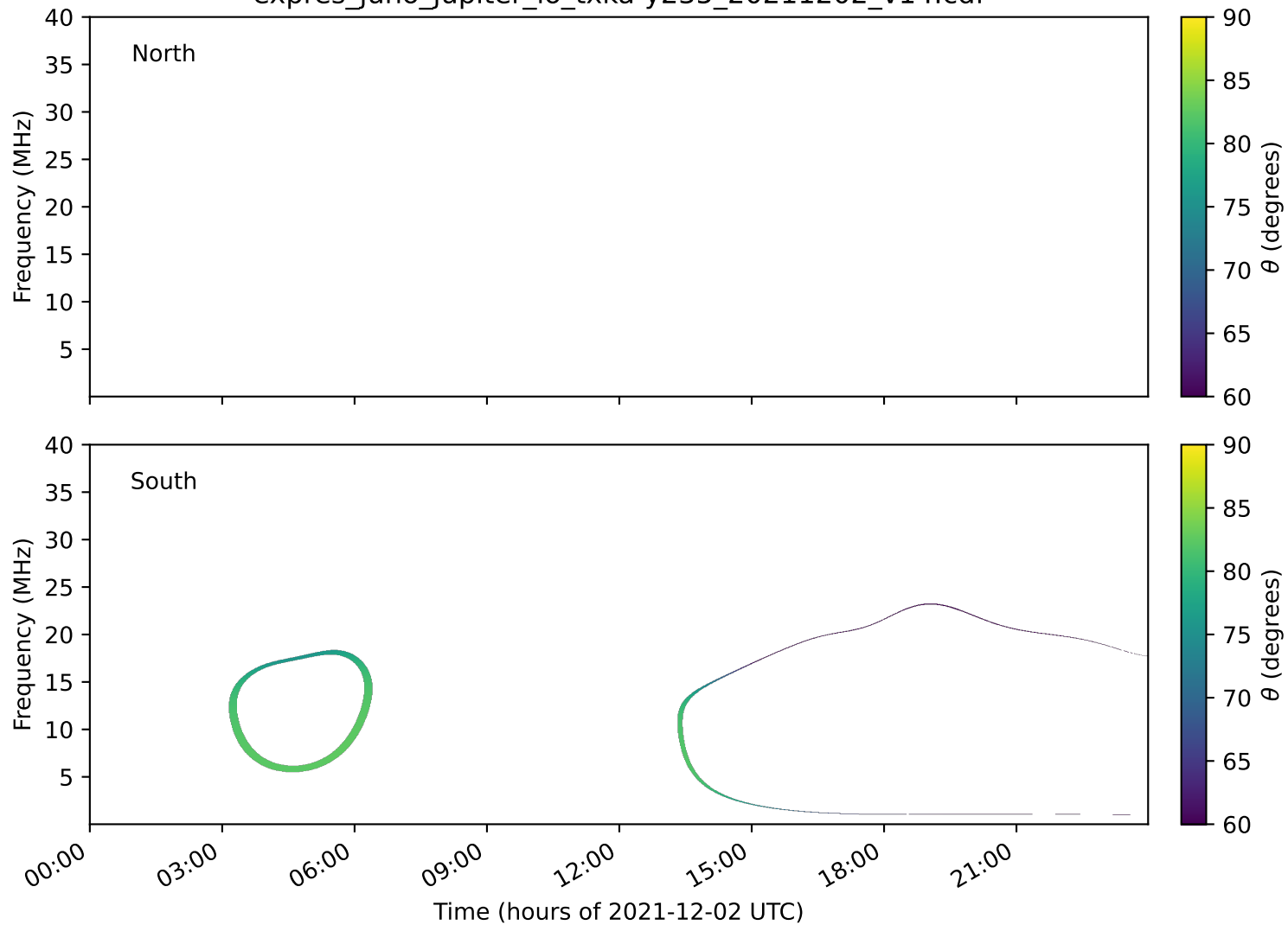
expres_juno_jupiter_io_txka-y235_20211202_v14.cdf
