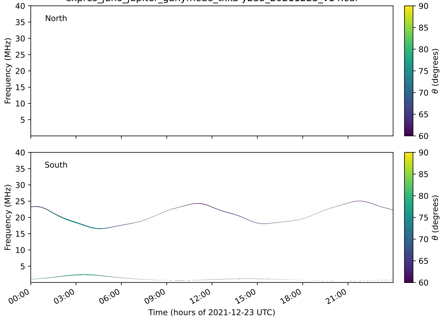
expres_juno_jupiter_ganymede_txka-y235_20211223_v14.cdf
