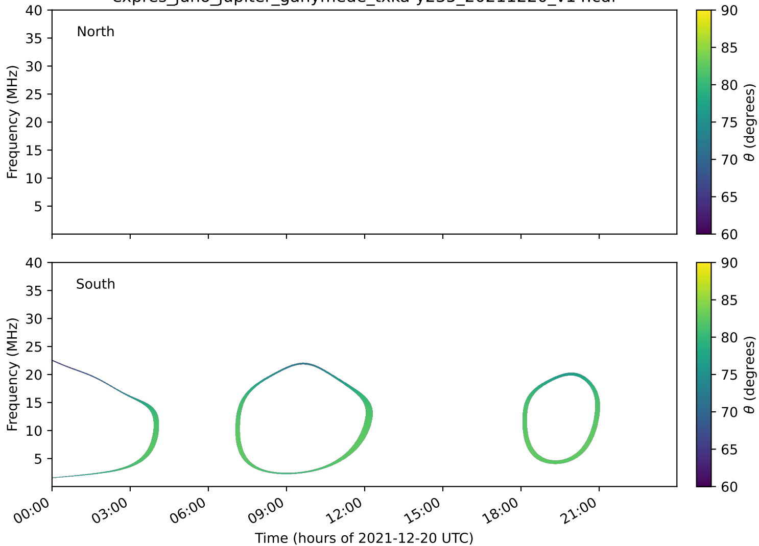
expres_juno_jupiter_ganymede_txka-y235_20211220_v14.cdf
