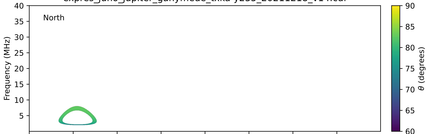
expres_juno_jupiter_ganymede_txka-y235_20211218_v14.cdf
