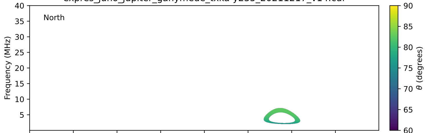
expres_juno_jupiter_ganymede_txka-y235_20211217_v14.cdf
