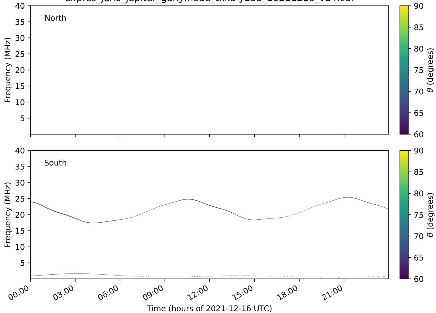
expres_juno_jupiter_ganymede_txka-y235_20211216_v14.cdf
