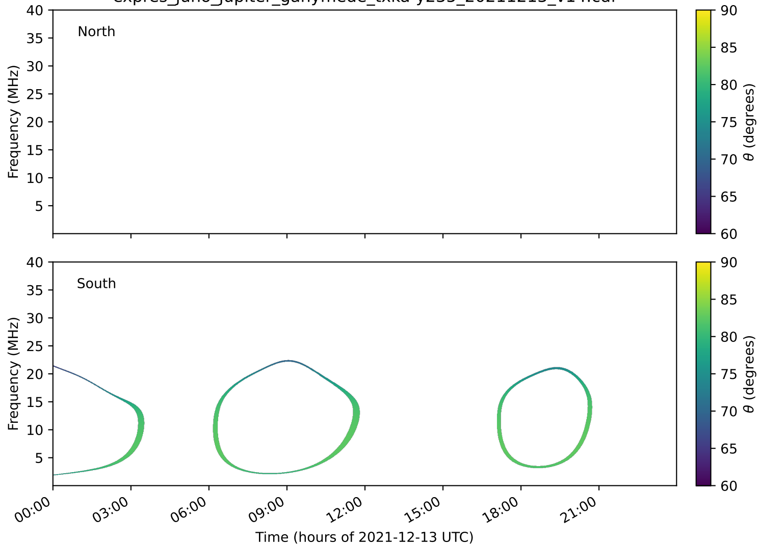
expres_juno_jupiter_ganymede_txka-y235_20211213_v14.cdf
