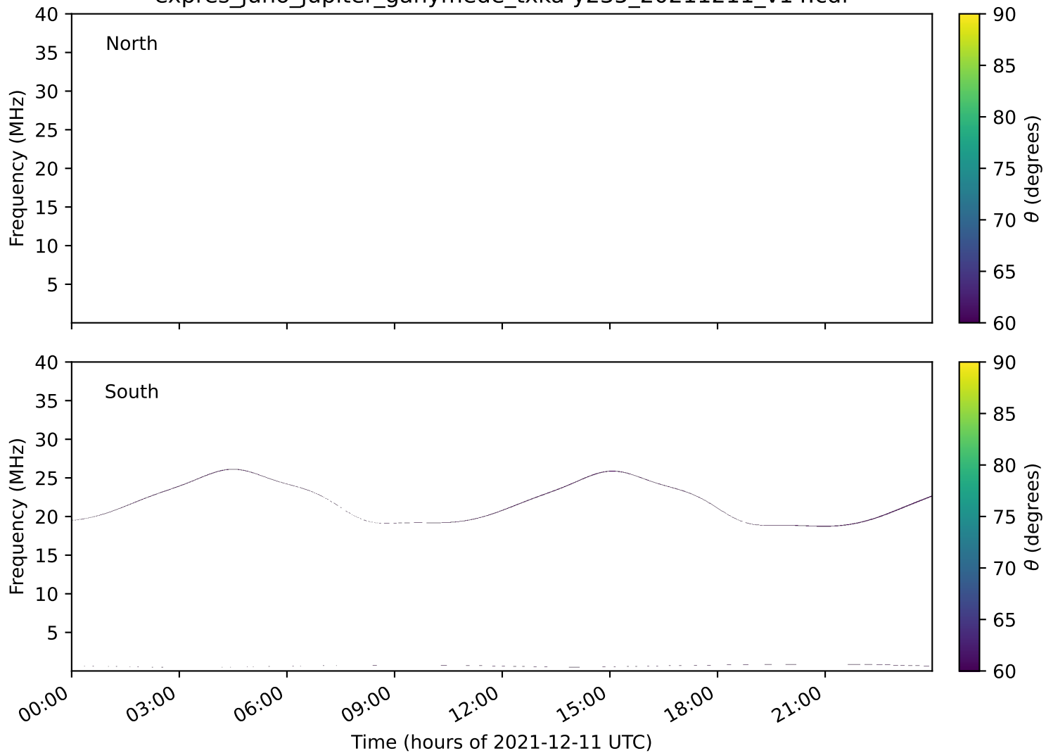
expres_juno_jupiter_ganymede_txka-y235_20211211_v14.cdf
