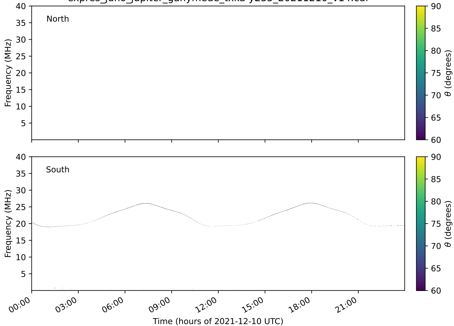
expres_juno_jupiter_ganymede_txka-y235_20211210_v14.cdf
