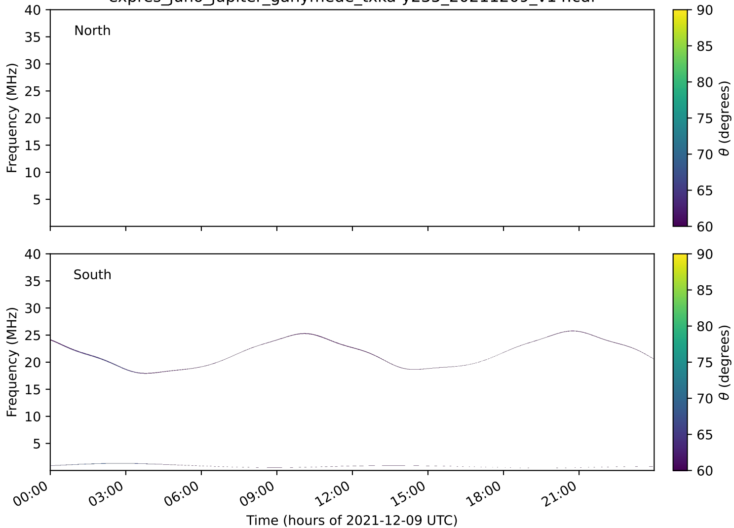
expres_juno_jupiter_ganymede_txka-y235_20211209_v14.cdf
