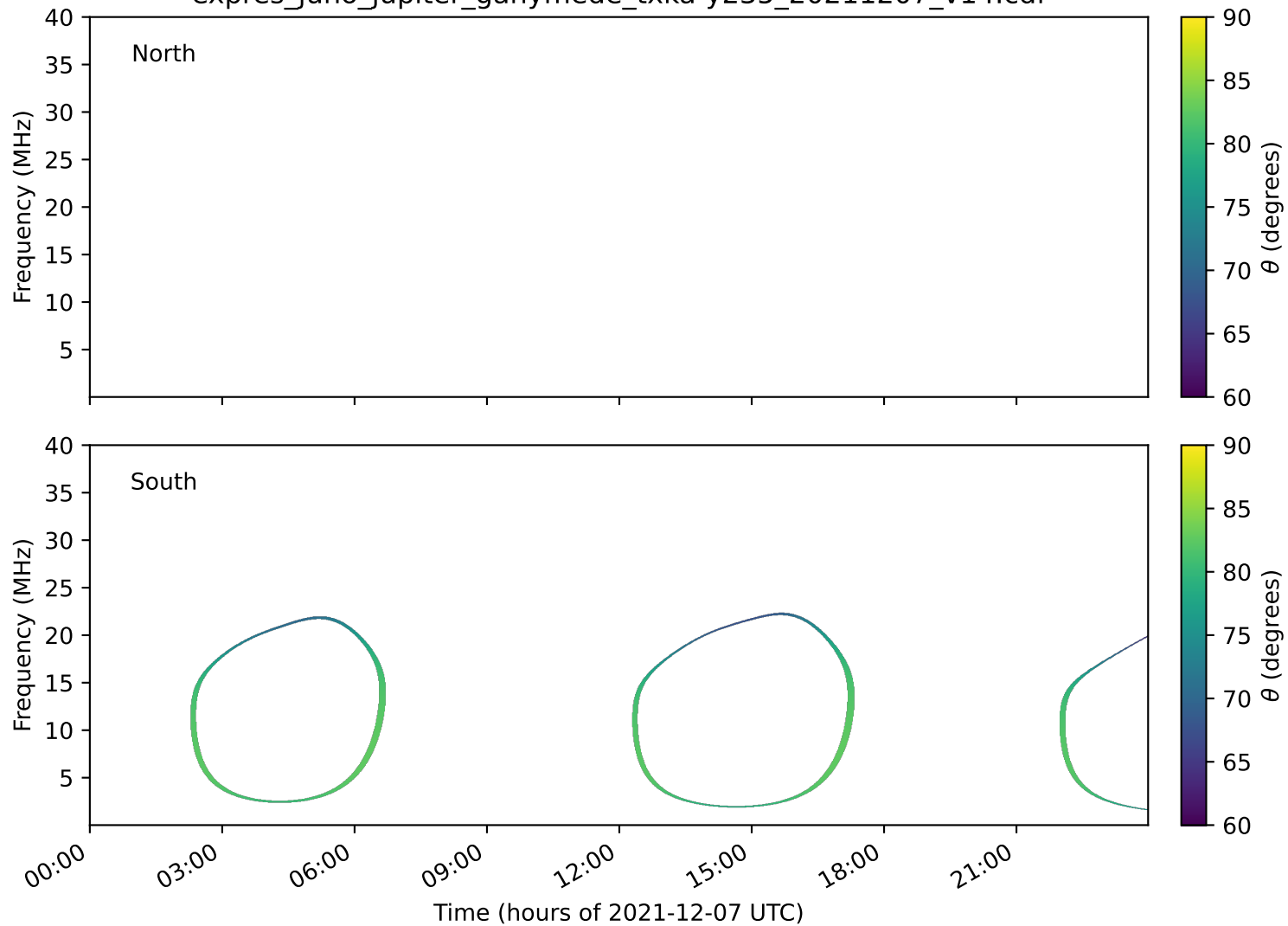
expres_juno_jupiter_ganymede_txka-y235_20211207_v14.cdf
