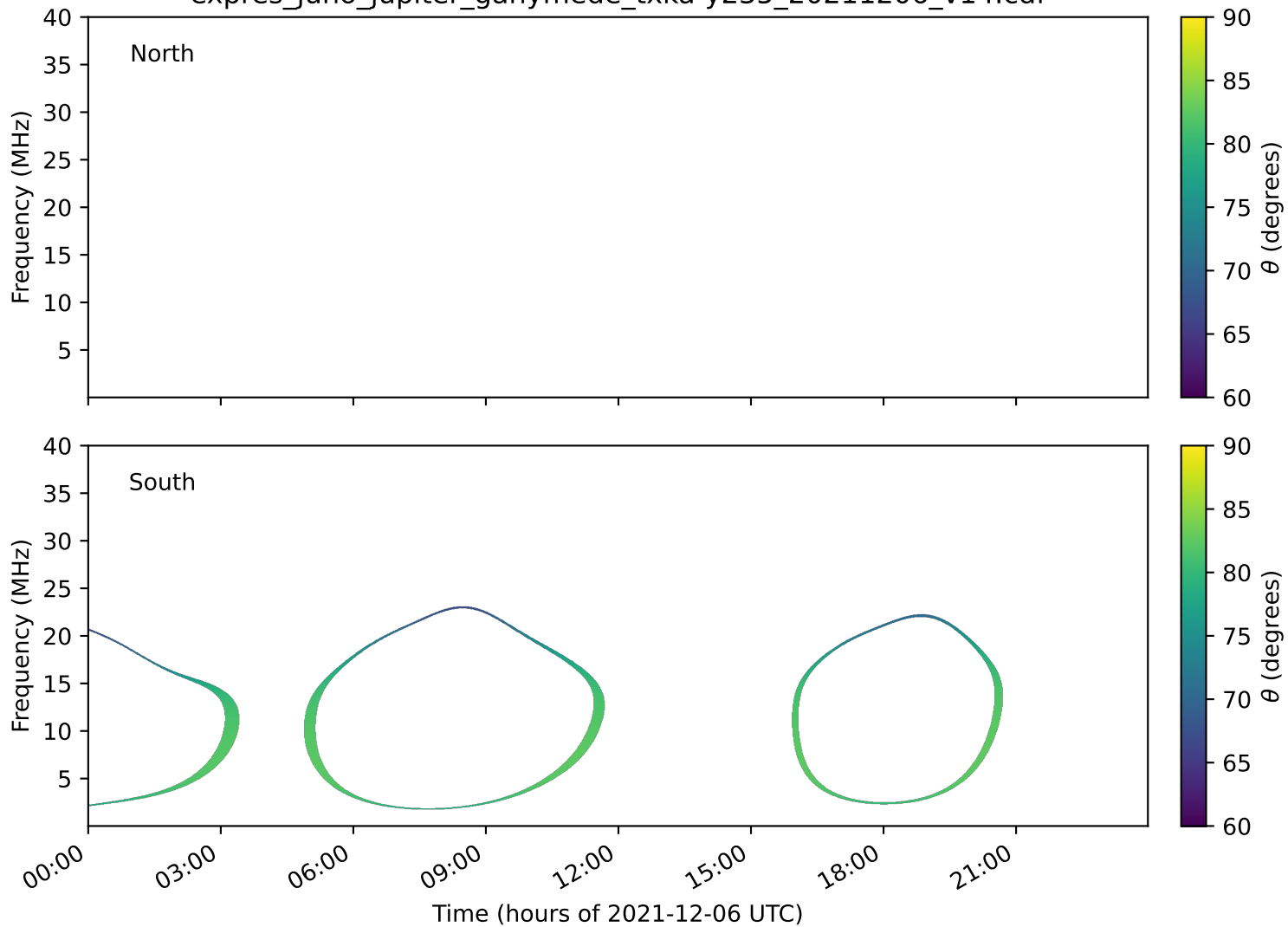
expres_juno_jupiter_ganymede_txka-y235_20211206_v14.cdf
