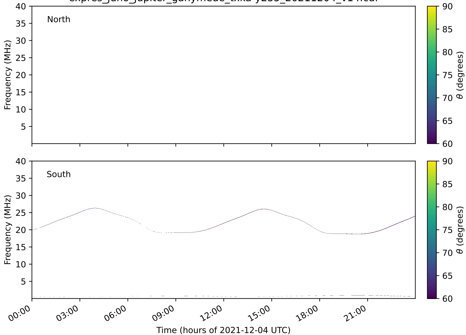
expres_juno_jupiter_ganymede_txka-y235_20211204_v14.cdf
