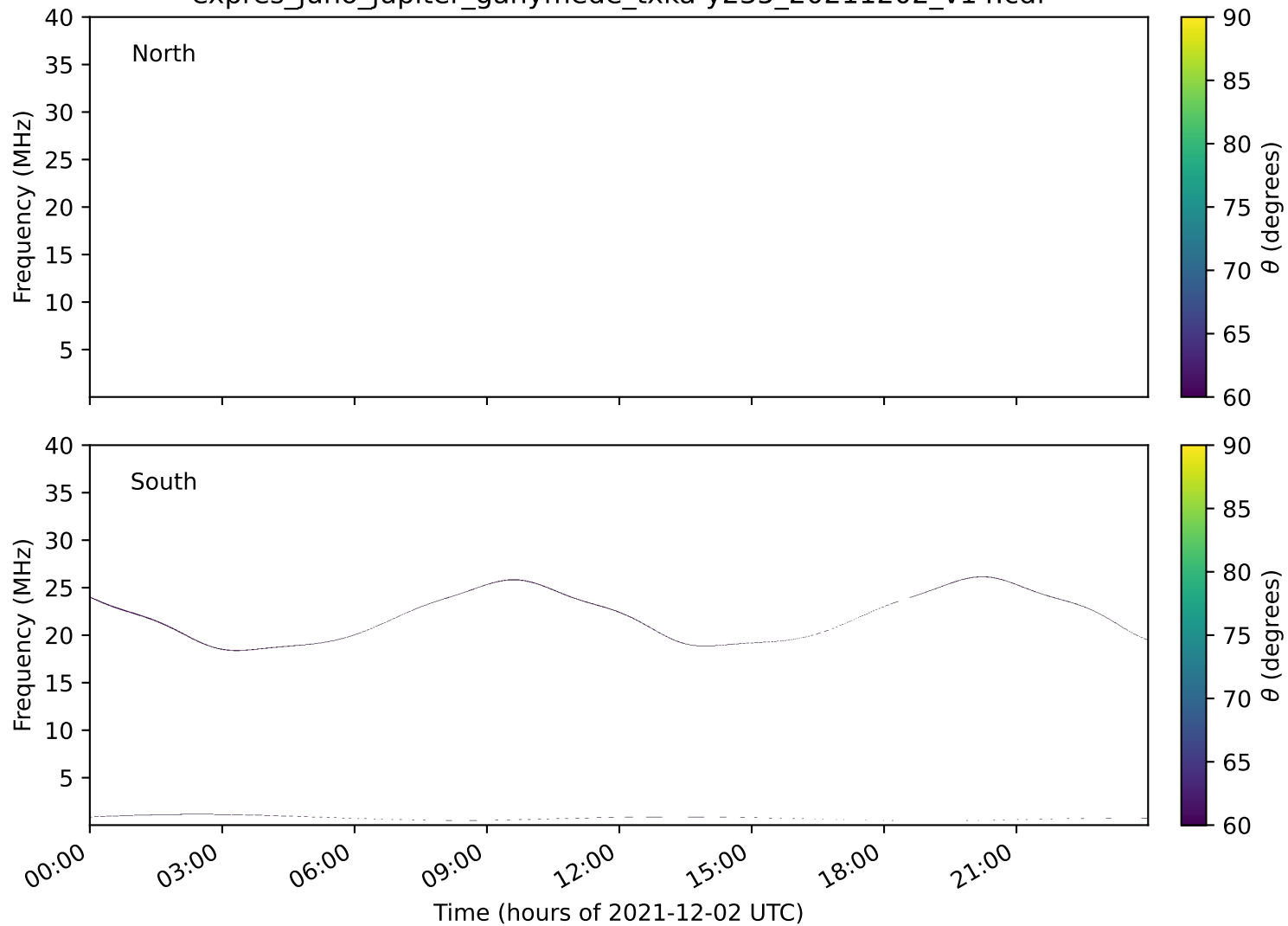
expres_juno_jupiter_ganymede_txka-y235_20211202_v14.cdf
