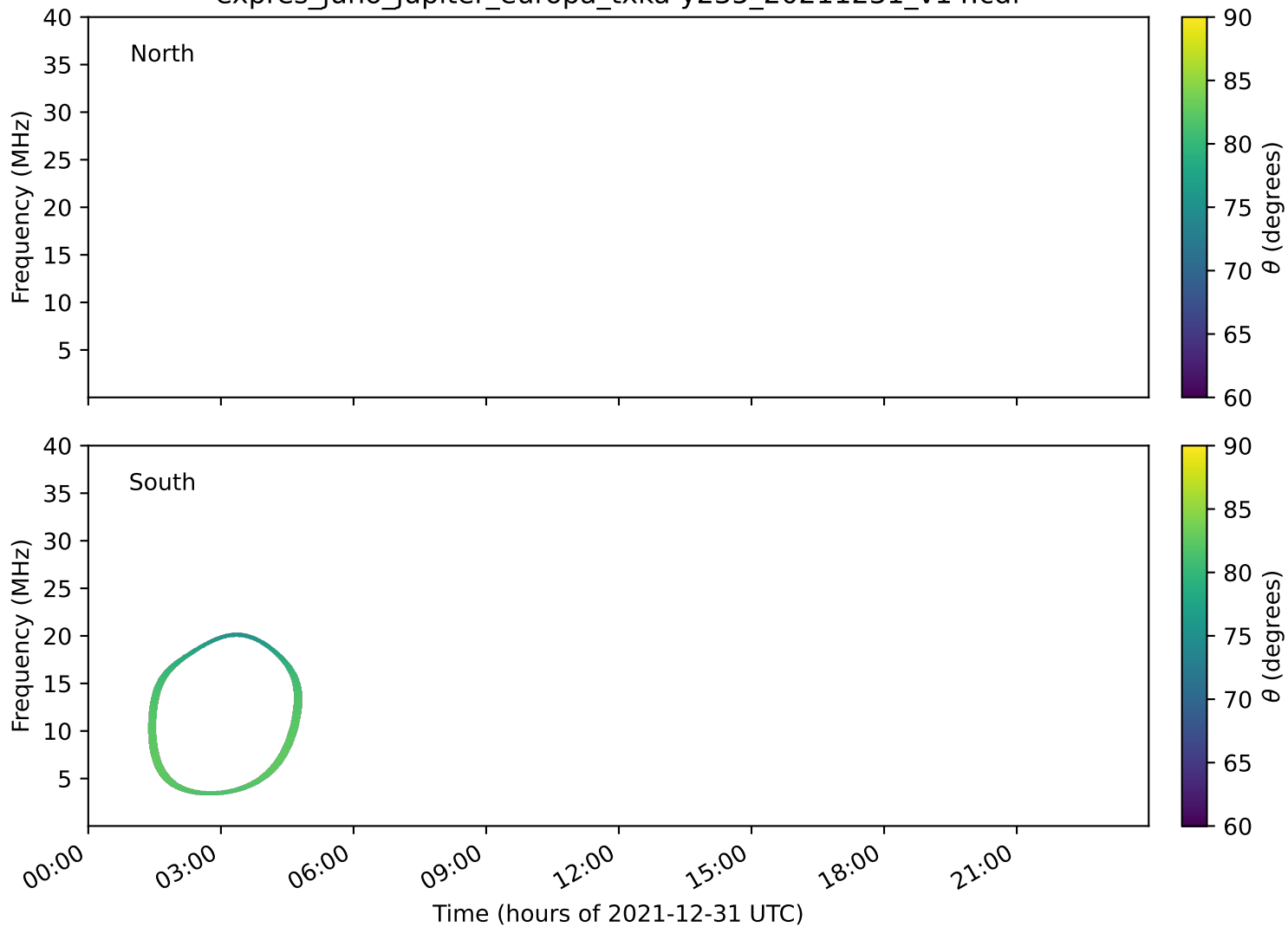
expres_juno_jupiter_europa_txka-y235_20211231_v14.cdf
