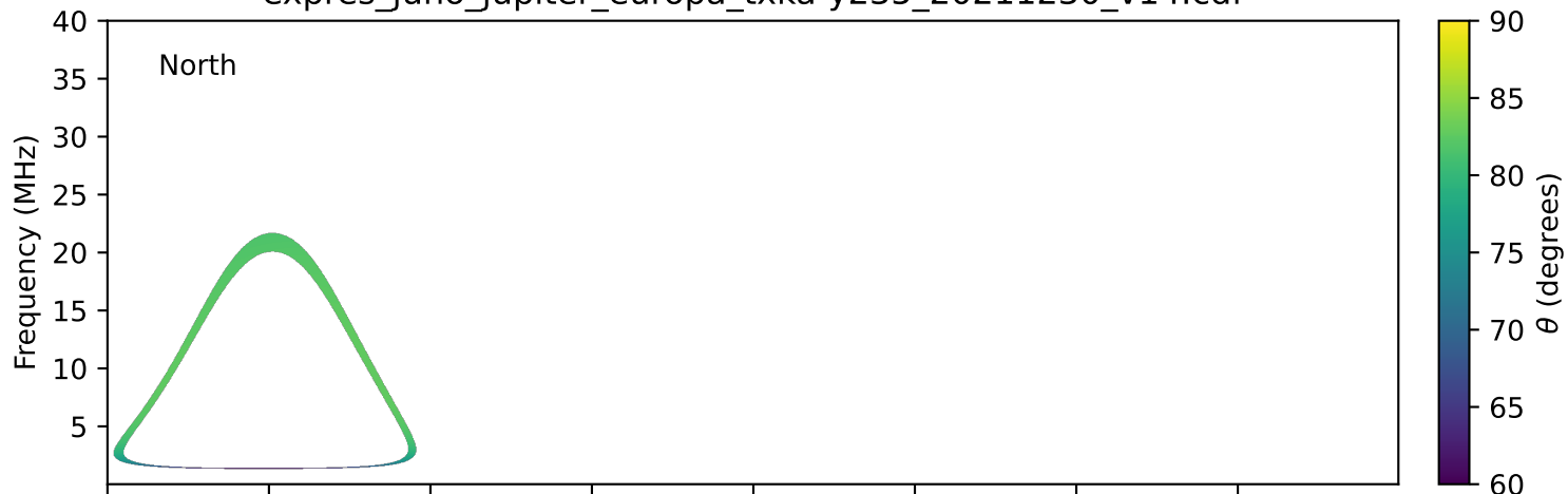
expres_juno_jupiter_europa_txka-y235_20211230_v14.cdf
