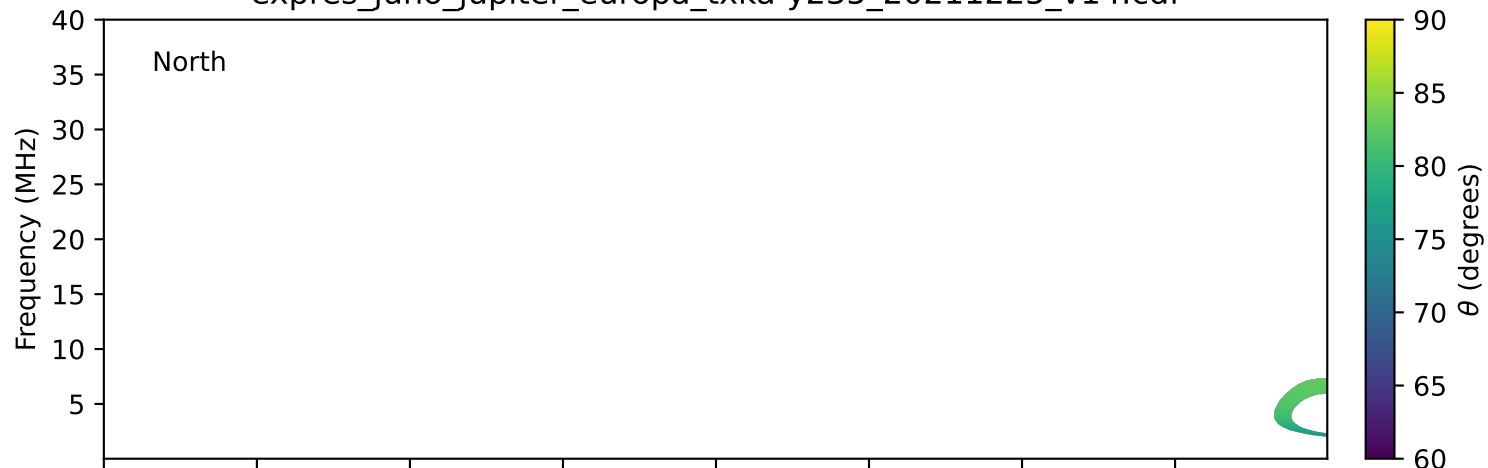
expres_juno_jupiter_europa_txka-y235_20211225_v14.cdf
