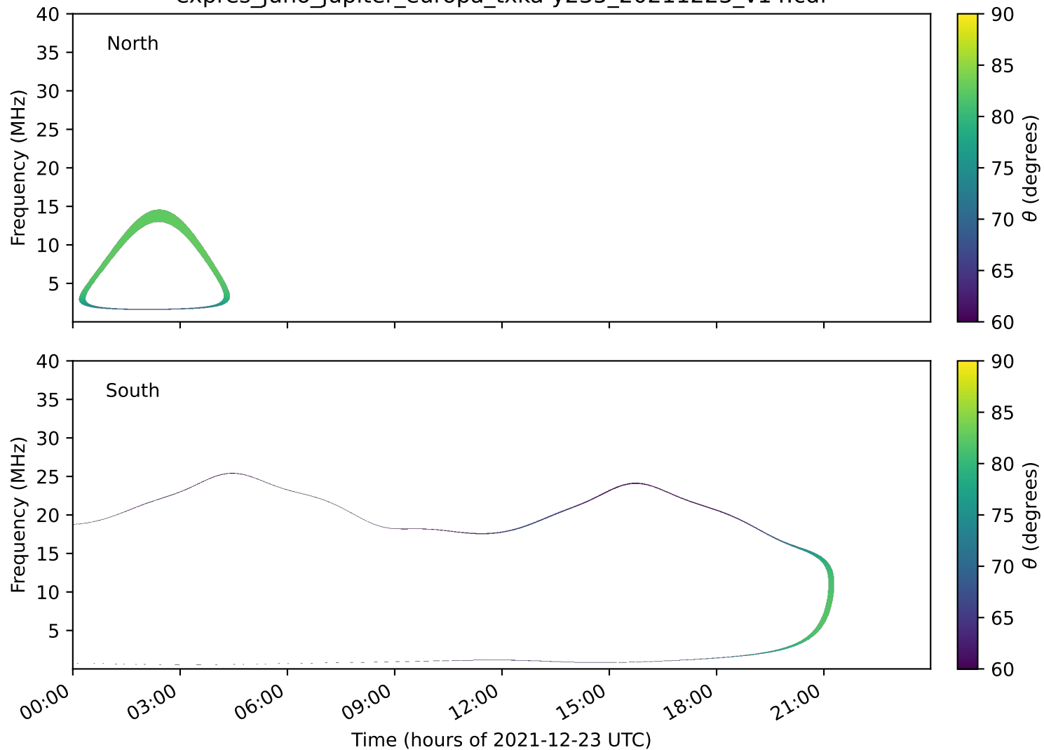
expres_juno_jupiter_europa_txka-y235_20211223_v14.cdf
