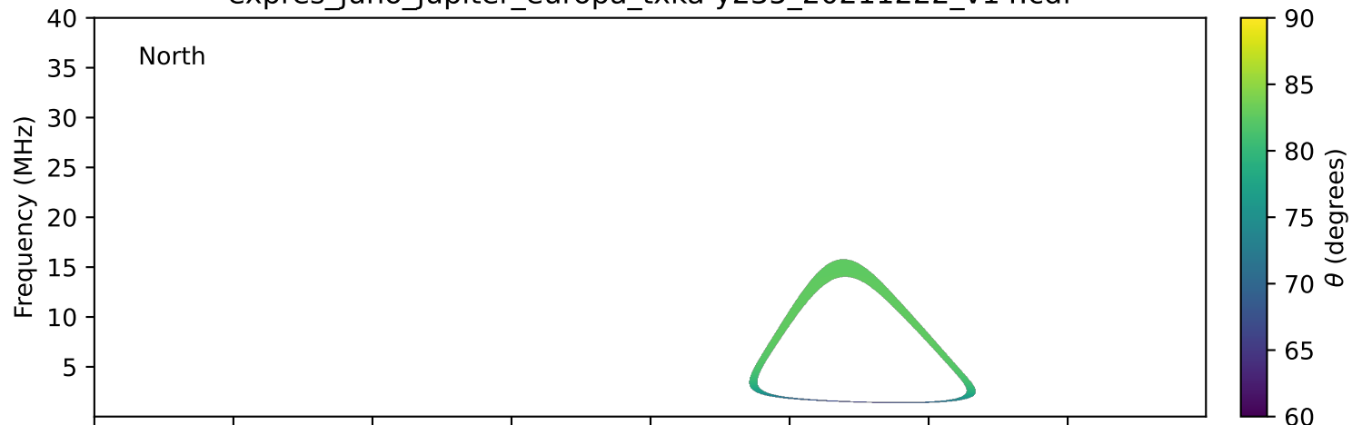
expres_juno_jupiter_europa_txka-y235_20211222_v14.cdf
