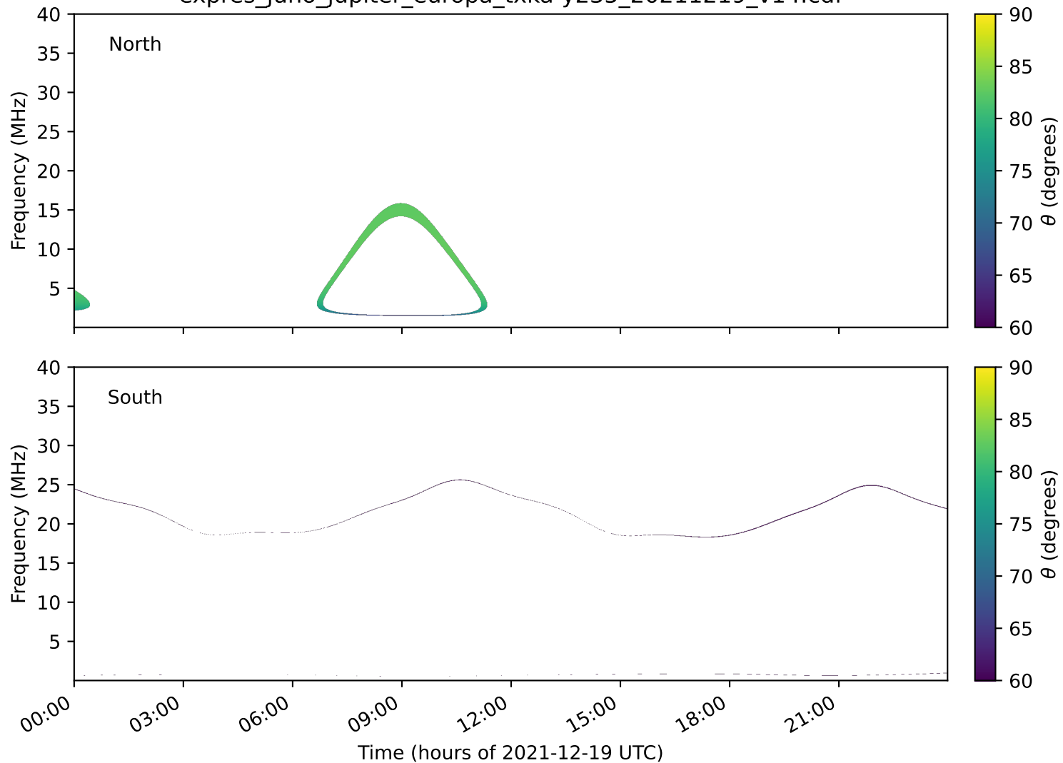
expres_juno_jupiter_europa_txka-y235_20211219_v14.cdf
