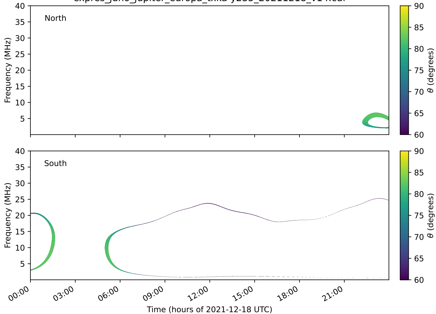
expres_juno_jupiter_europa_txka-y235_20211218_v14.cdf
