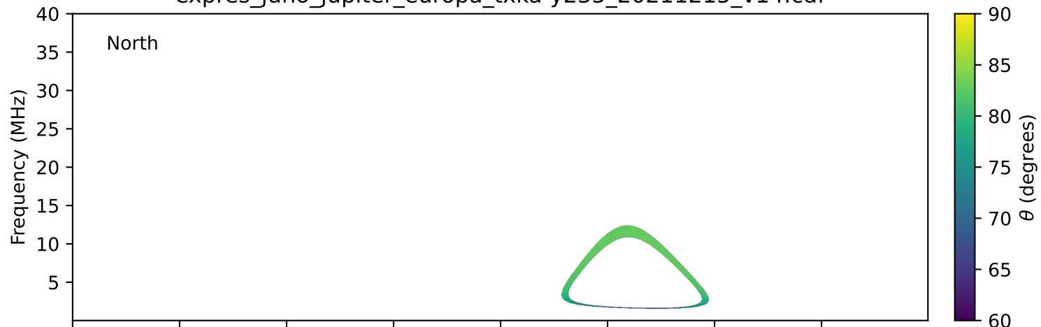
expres_juno_jupiter_europa_txka-y235_20211215_v14.cdf
